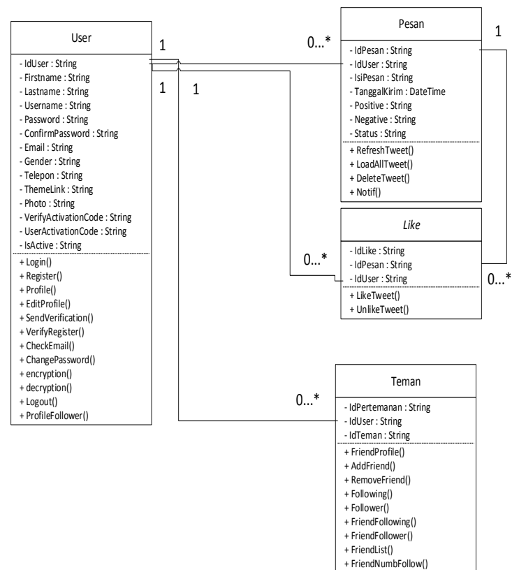
Gambar 4 Class Diagram Sistem
