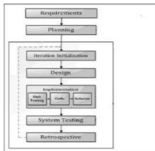
Gambar 2 Alur Kerja Personal Extreme Programming
