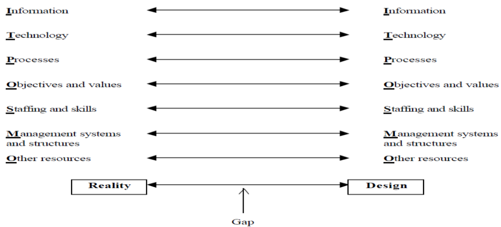
Gambar 2. Framework ITPOSMO
