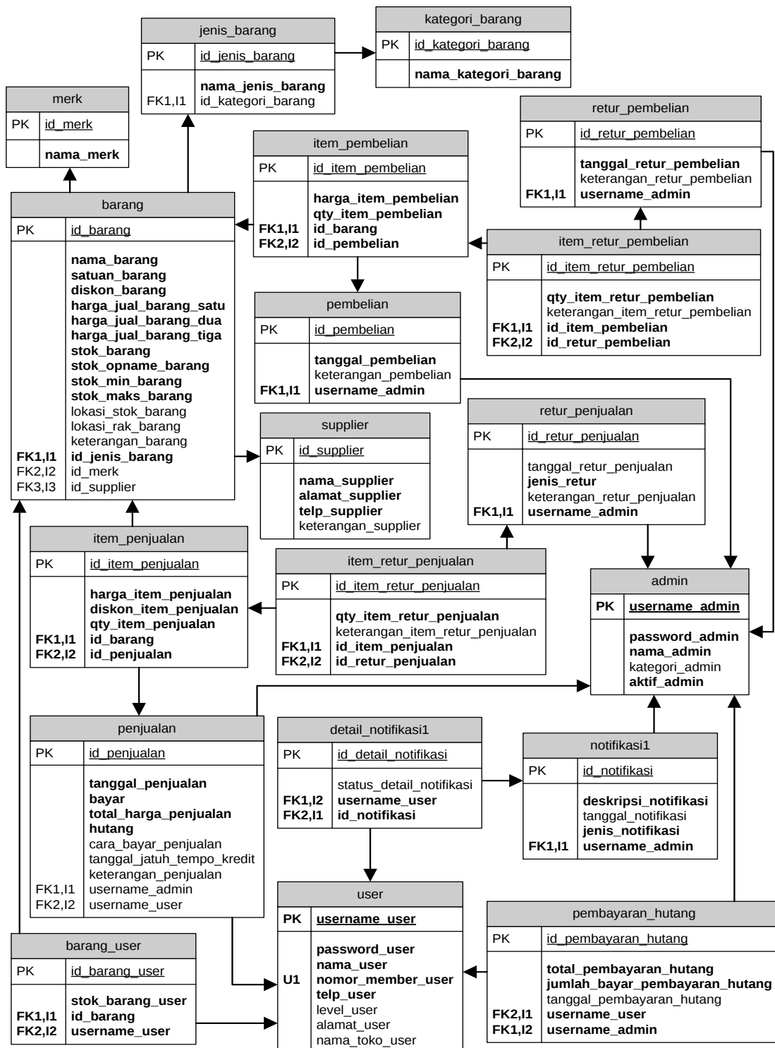
Gambar 5 Entity Relationship Diagram (ERD)
