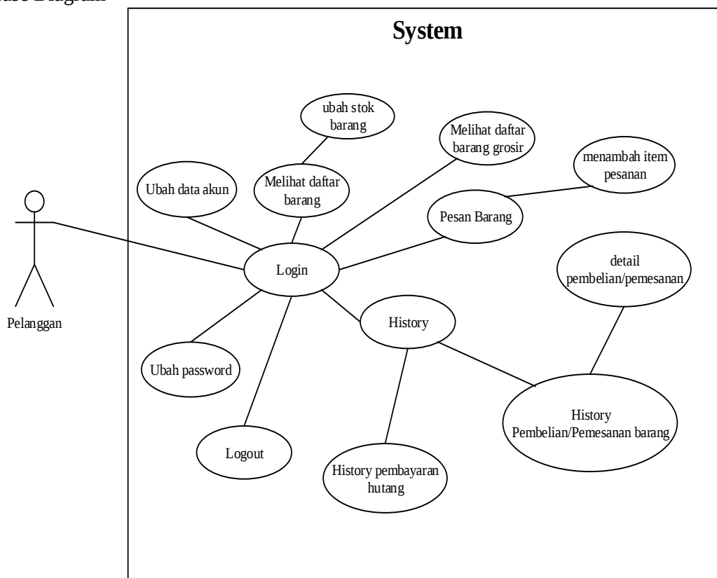
Gambar 3 Use Case Diagram Pelanggan
