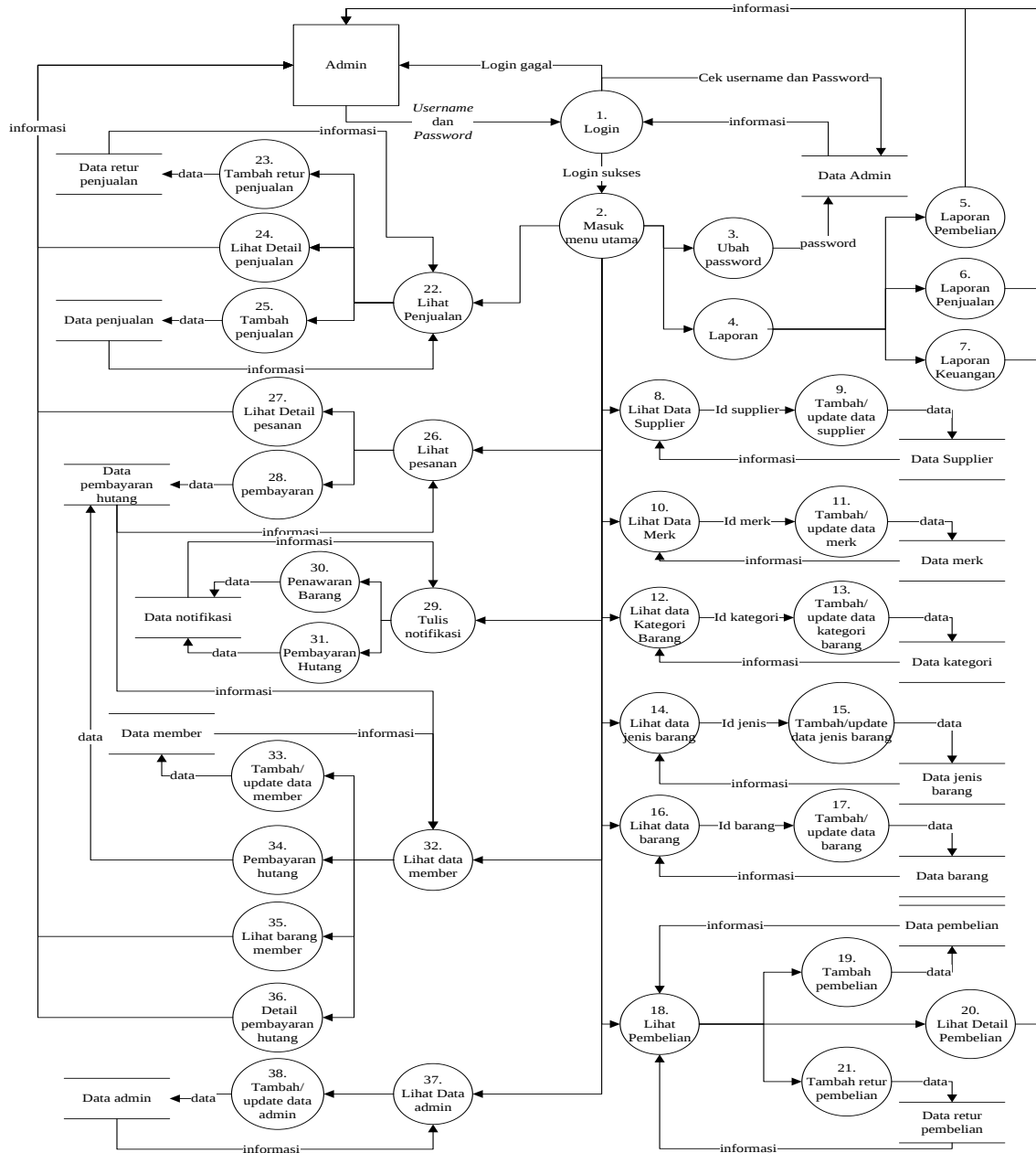
Gambar 1 DFD Admin Level 1
